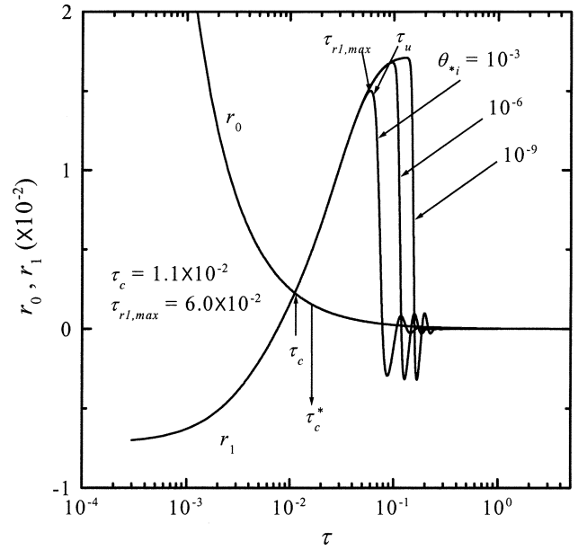
Fig. 7. Comparison of growth rate of mean temperature with its perturbed one for \theta_{si}=10^{-3}, 10^{-6}, 10^{-9} with Ra=10^4 and a_c=4.5 .
