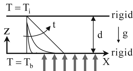
Fig. 1. Schematic diagram of conduction state considered in the present study.
